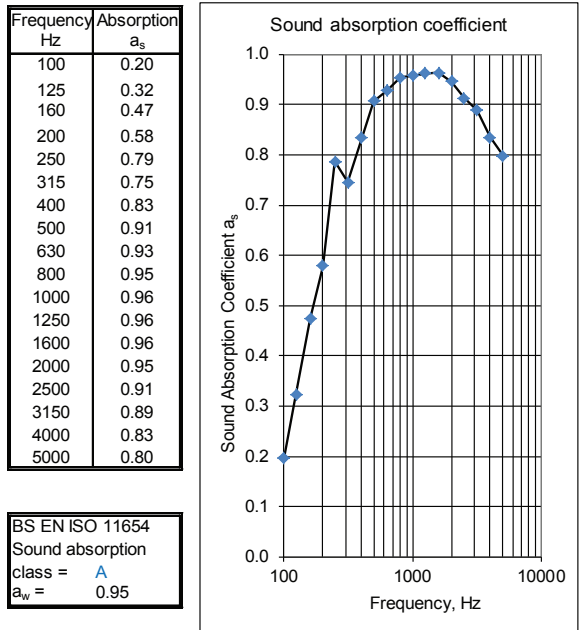
50mm system
